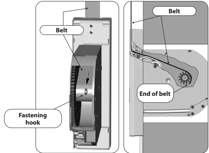
Belt path in RolloTron Comfort DuoFern
