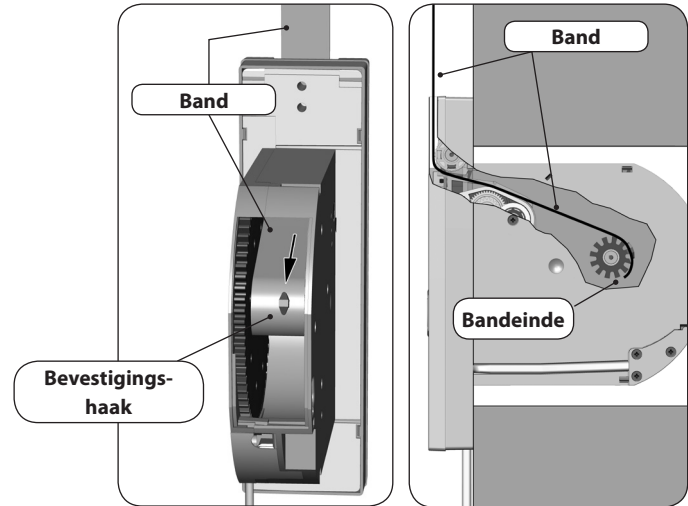
Bandverloop in de RolloTron Standard
