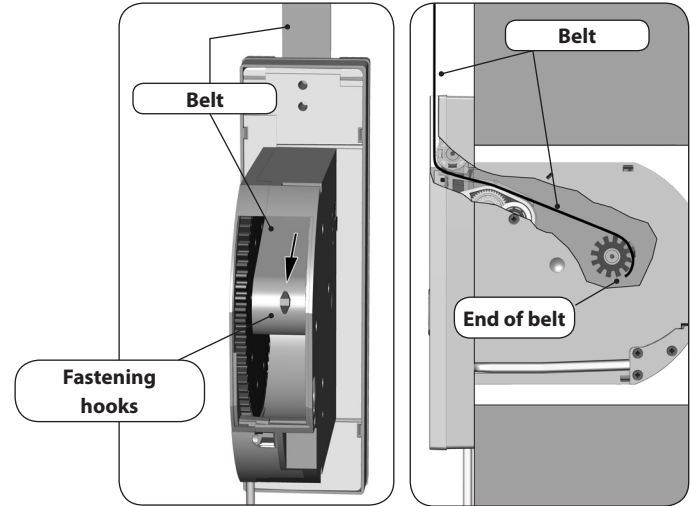
Belt path in RolloTron Standard
